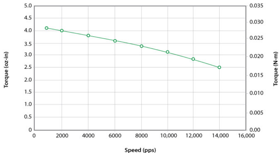
3809Y-51 24VDC, 0.6 Amps/Phase, Bipolar, 1/2 Stepping
